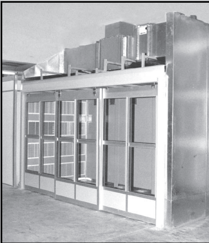
Self-contained mechanical equipment furnishes constant temperature and air flow for testing of communication equipment.
