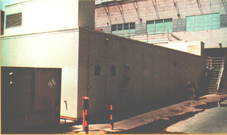
Acoustical enclosure with "single pass" silenced ventilation system.
